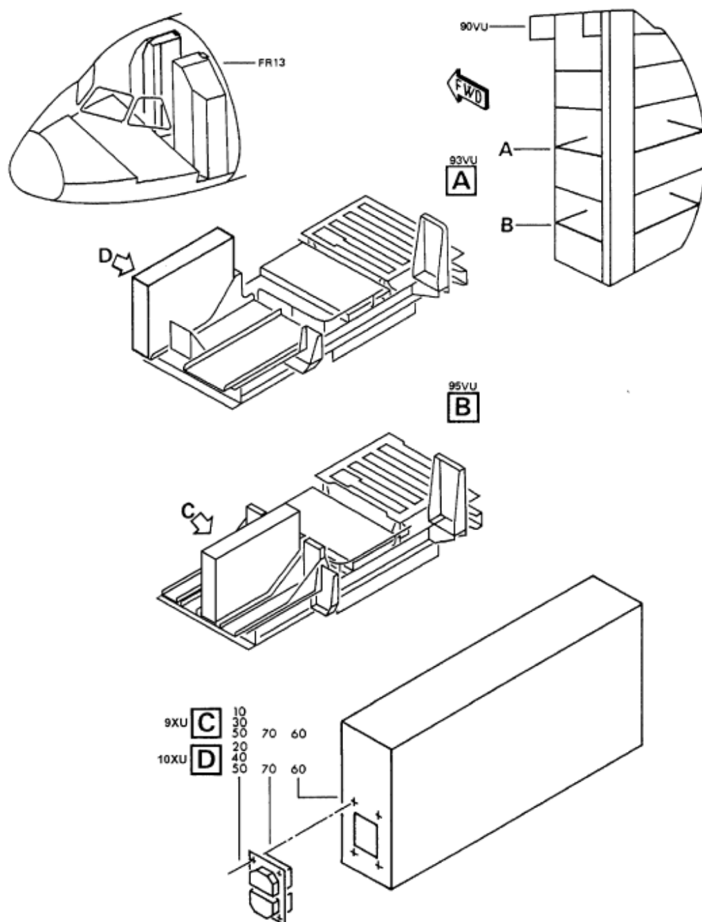
EQUIPMENT INSTL, Z213-214 Figure 02
