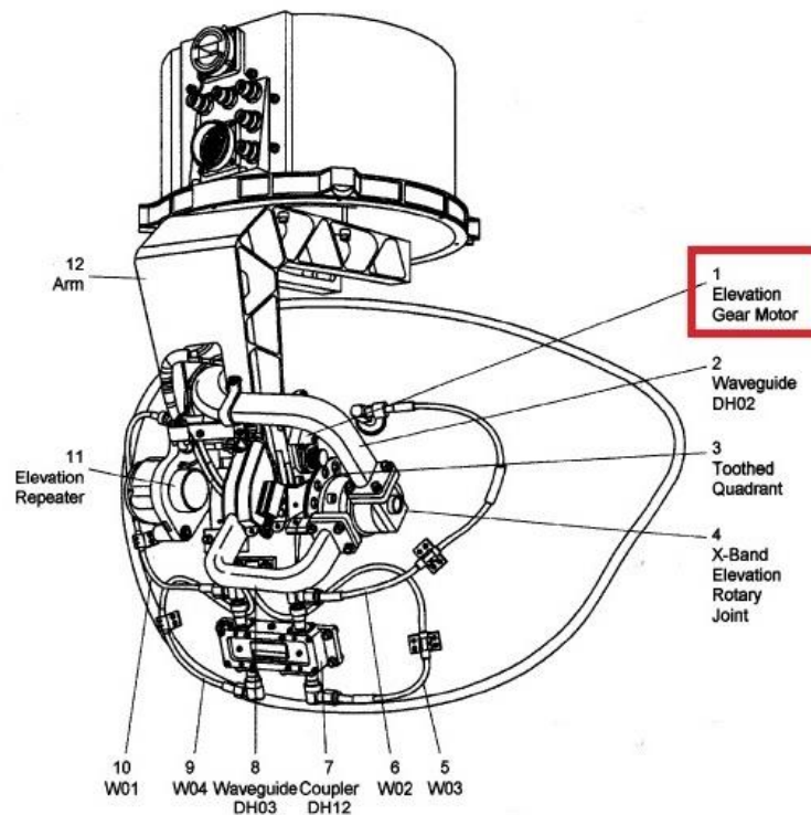
Figure 4 Radar Antenna - Overview on reflector backside
