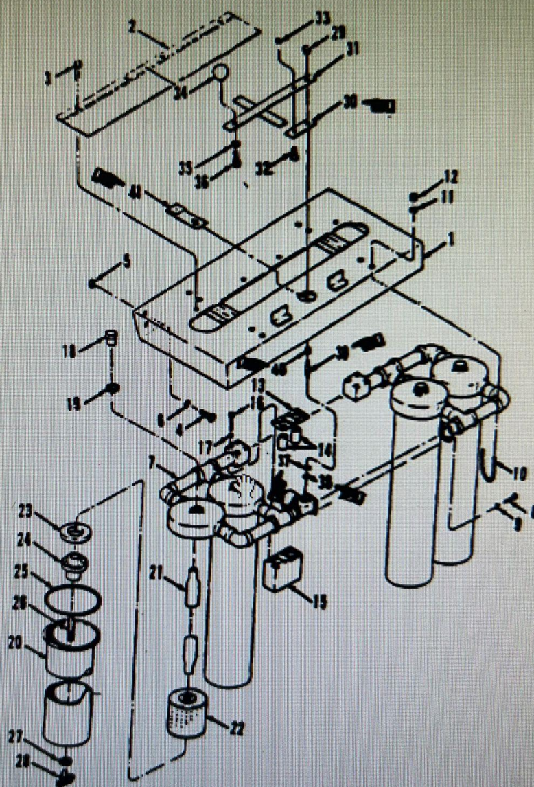
Figure 2-2-3. Fuel Filter Assembly
