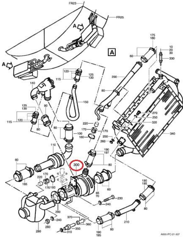
ENVIRONMENTAL CTL UNIT INSTL, Z191-192 Figure 70C
