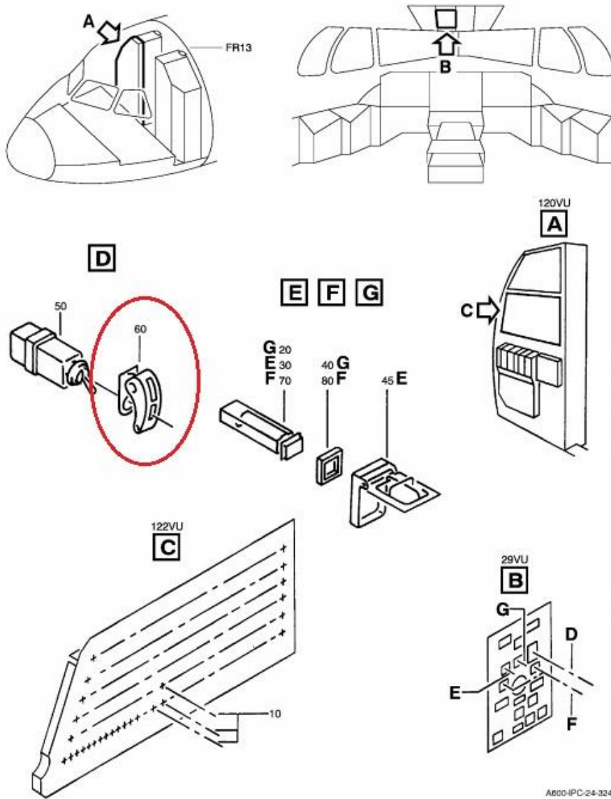
EQUIPMENT INSTL, Z211-212 Figure 04A
