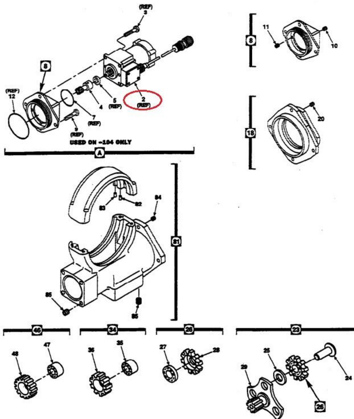
Figure 11. Main Rotor Blade Fold Actuator (Sheet 2)
