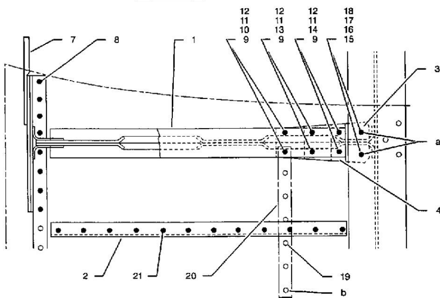
Installation details Figure 801
