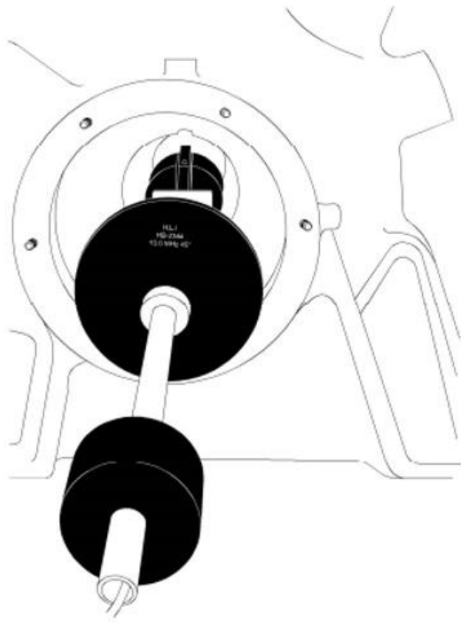
Figure 3-7H – Ultrasonic Inspection Tool in Output Bevel Gear Bore
