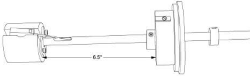
Figure 3-7B – Ultrasonic Inspection Tool I
