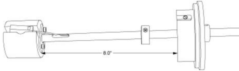
Figure 3-7C – Ultrasonic Inspection Tool II
