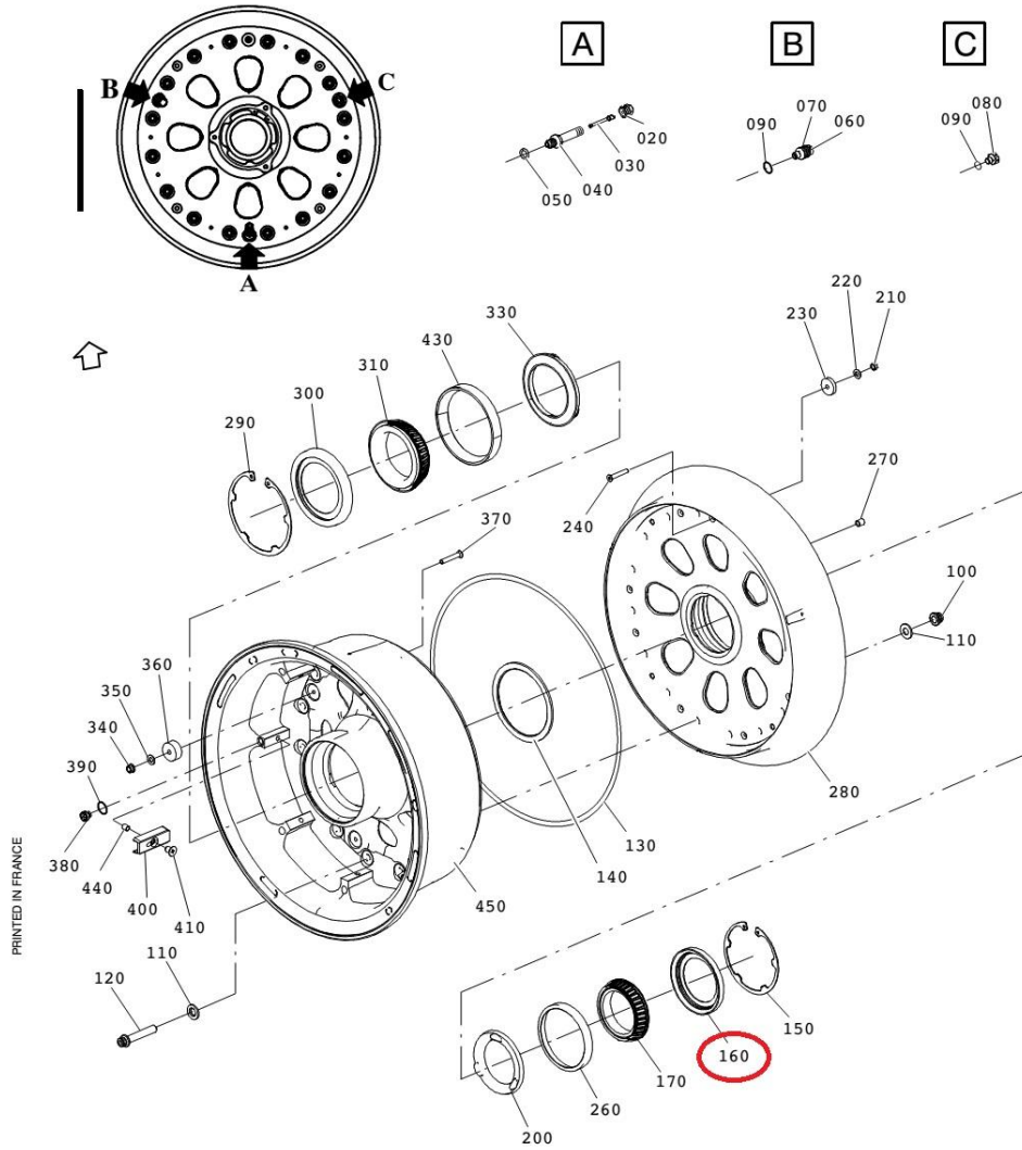
Exploded view of the main landing gear wheel assembly Figure 1
