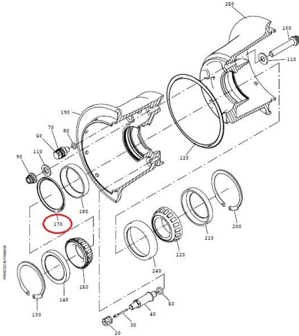
Exploded view of the nose wheel assembly Figure 1
